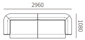
31F033-22R + 31F033-22L 2960*1080*670MM 116.5*42.5*26.4"
