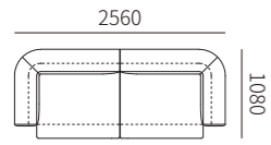
31F033-21R + 31F033-21L 2560*1080*670MM 100.8*42.5*26.4"
