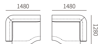
31F033-23AR 31F033-23AL 1480*1280*670MM 58.3*50.4*26.4"
