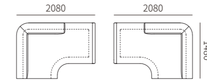
31F033-42L 31F033-42R 2080*1480*670MM 81.9*58.3*26.4"
