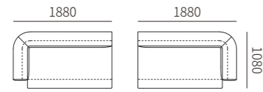
31F033-25R 31F033-25L 1880*1080*670MM 74.0*42.5*26.4"
