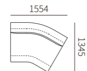
31F033-33 1554*1345*670MM 61.2*53.0*26.4"
