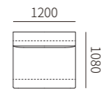
31F033-32 1200*1080*670MM 47.2*42.5*26.4"
