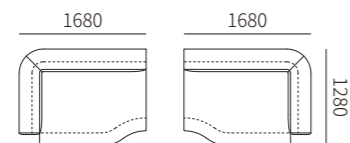
31F033-24AR 31F033-24AL 1680*1280*670MM 66.1*50.4*26.4"
