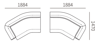
31F033-27R 31F033-27L 1884*1470*670MM 74.2*57.9*26.4"
