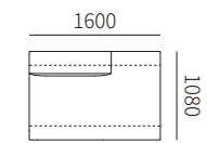
31F033-71 1600*1080*670MM 63.0*42.5*26.4"
